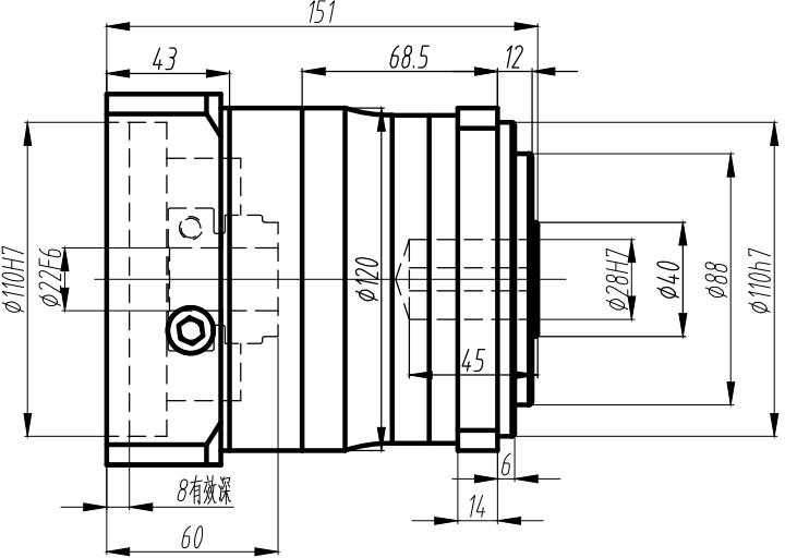
标准轴 Standard output shaft
