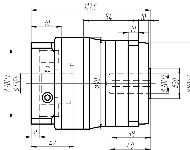
标准轴 Standard output shaft
