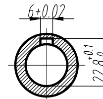
标准轴 Standard output shaft
