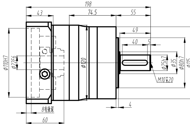
标准轴 Standard output shaft
