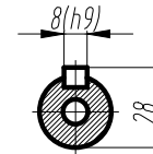
标准轴 Standard output shaft
